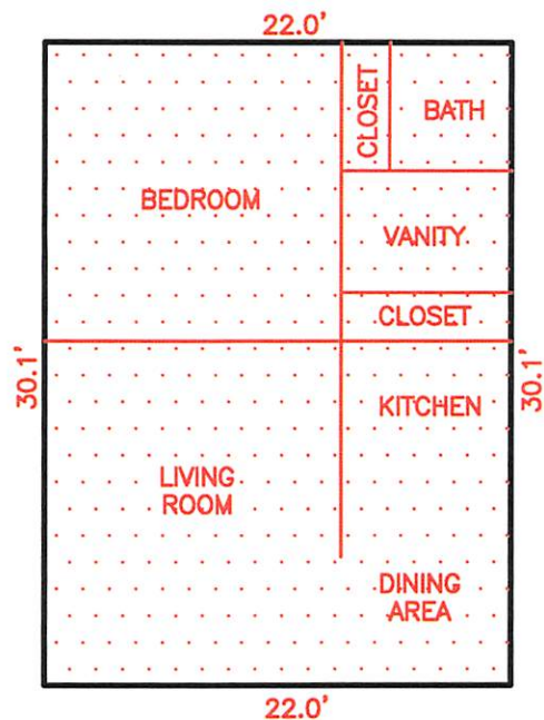
UNIT 82 TYPICAL ONE BEDROOM ONE BATH UNIT 662 s.f.
